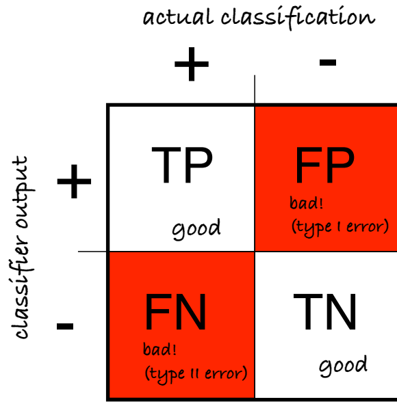
Figure 1: Confusion matrix for a binary classifier which maps the true classification against the output of the classifier.
